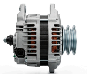
ALTERNADOR Mazda BT 50 12V (70AMP)
